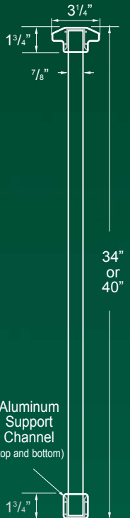
"A" Series Decorative Spindle Railing End View
